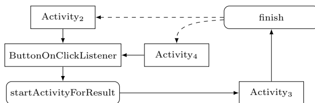
Figure 9: The problem of using path matching approach for startActivityResult
