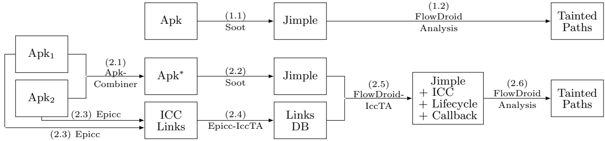
Figure 4: Overview of IccTA (down) and FlowDroid (up).
